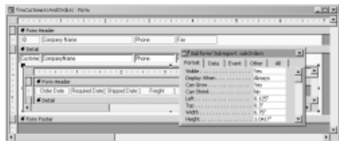
Figure 5. Design view of a form with an expanding subform.
